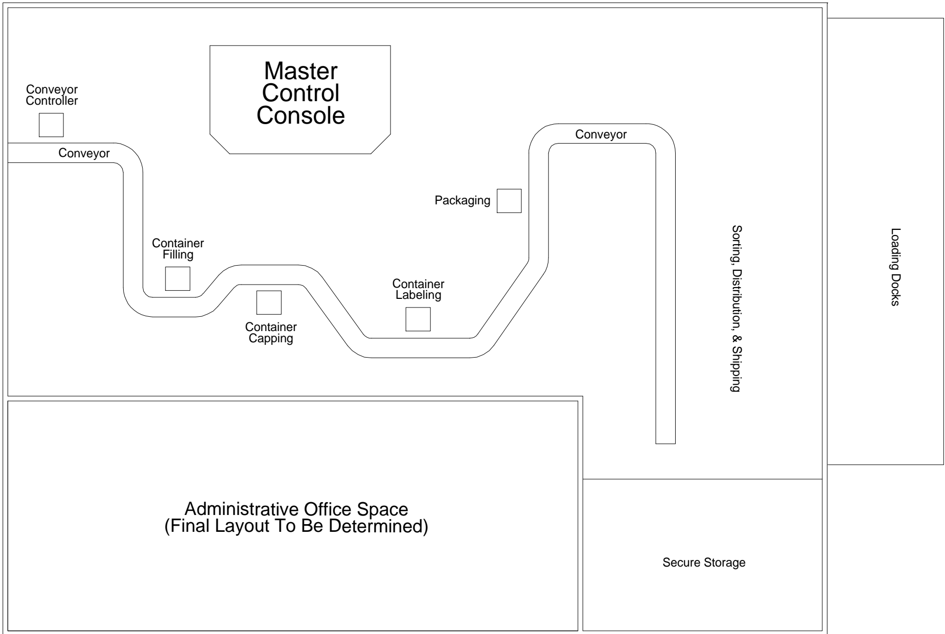
Apache Facility Expansion Automated System Expansion Conceptual/Schematic Layout
