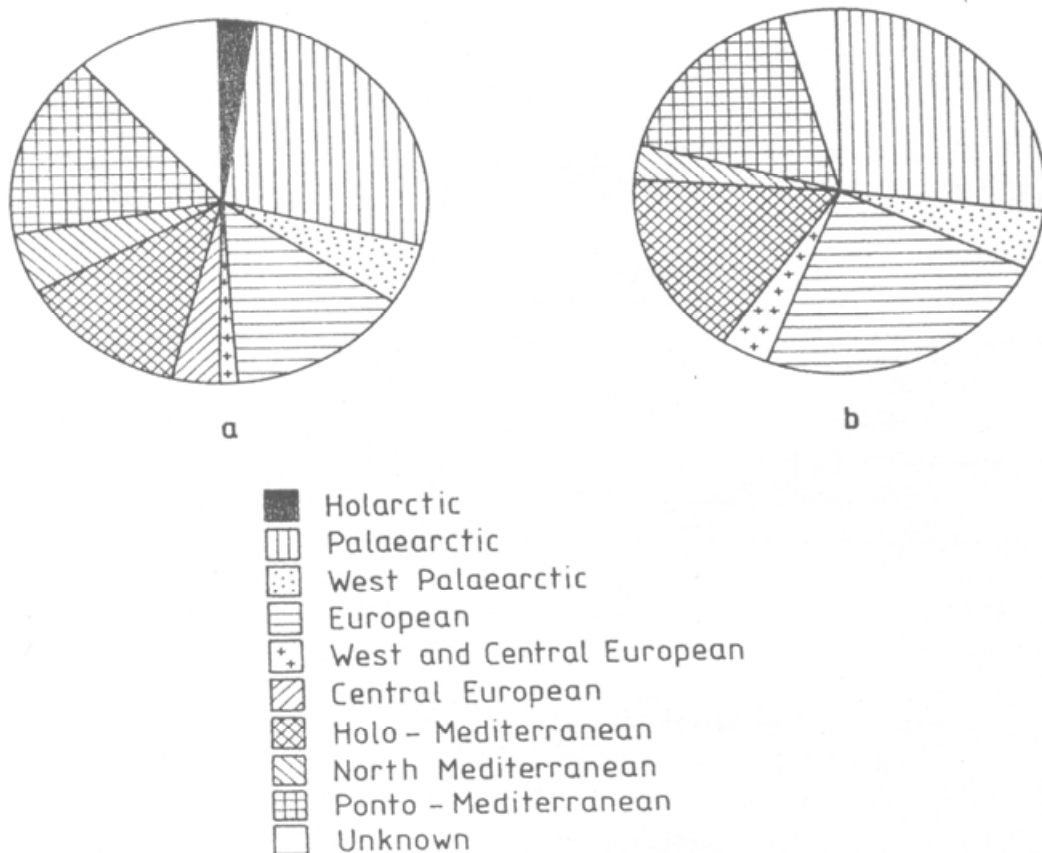
Fig. 1: Distribution of Sphecid assemblage according to zoogeographical distribution: a: all species, b: weighted on basis of relative frequency of sphecid species found in traps
