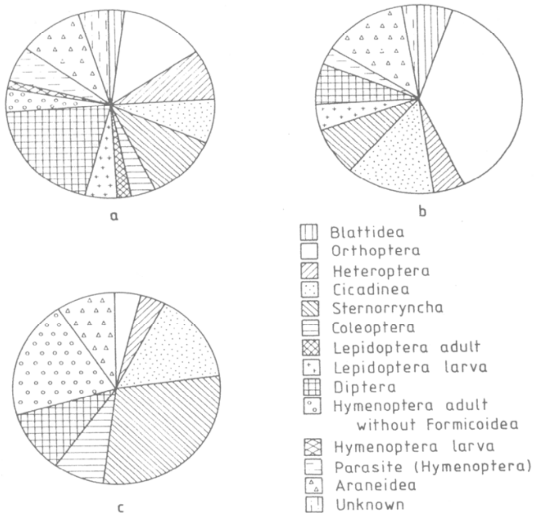
Fig. 3: Distribution of Sphecid assemblage according to prey species: a: all species, b: weighted on basis of relative frequency of sphecid species found in traps c: distribution of possible prey species (caught in pitfall traps)
