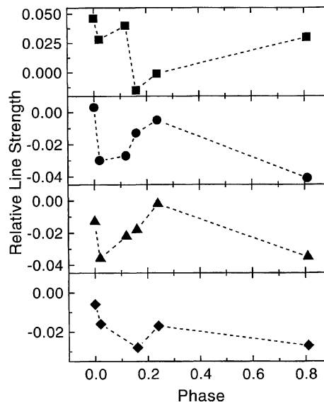
FIG. 5. Relative line strengths of H\alpha (filled square), Ca II lines at 8498 Å (circle), 8542 Å (triangle), and 8662 Å (diamond), as a function of light-variation phase. Variation in the Ca II lines at 8498 Å and 8542 Å mimic each other, whereas the Ca II line at 8662 Å does not follow the same trend.
